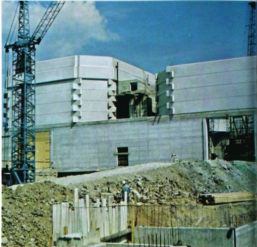
Fig. 12 Studios 2 and 3 during construction. The upper parts of the studio walls are reinforced-concrete sections assembled in log-cabin fashion.
