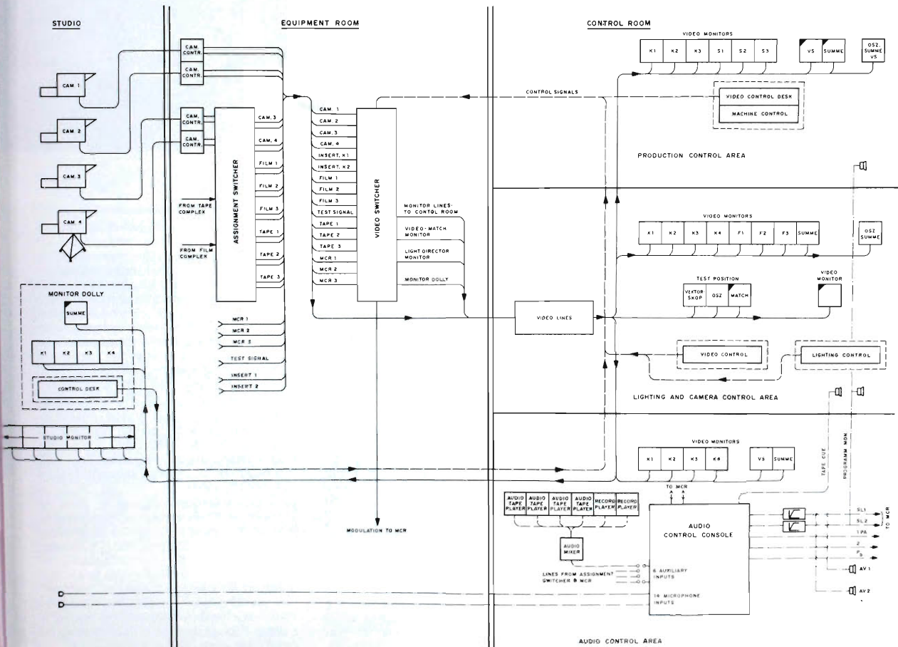
Fig. 22 Simplified video and control schematic showing divisions of equipment between studio, equipment room and control room for Studio 1, 2 or 3. Solid lines are video circuits, broken lines are audio circuits and dashed lines are control circuits.
