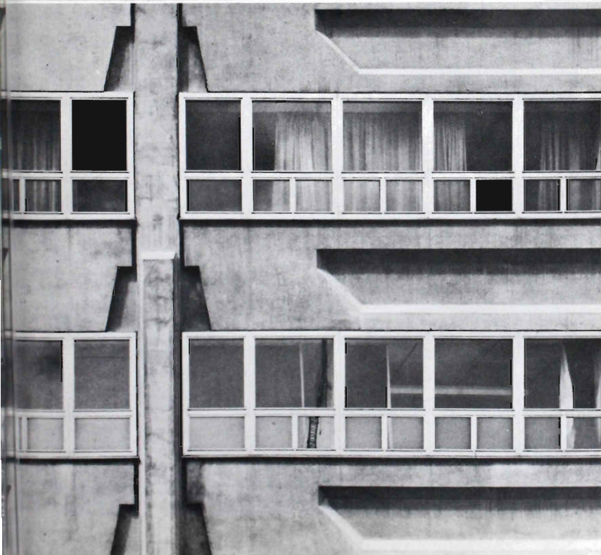
Fig. 11 The height of the girders is such that when assembled a single girder forms the wall from the top of one window to the bottom of the window above—thus eliminating individual window sills and other minor details. The length of the girders provides unusually wide spacing between interior pillars.
