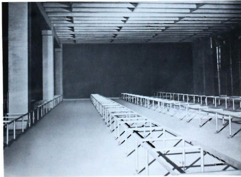
Fig. 26 The control equipment room before installation of the equipment racks which will rest on the frames seen here. Spaces between the frames will be filled with "computer-type" floor at the same level as the height of the frames. This will provide maximum convenience in installation and maintenance.
